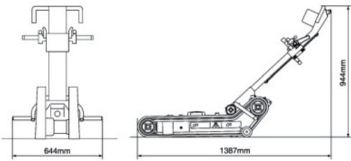
SCHEMAT TRANSPORTERA SA-S
