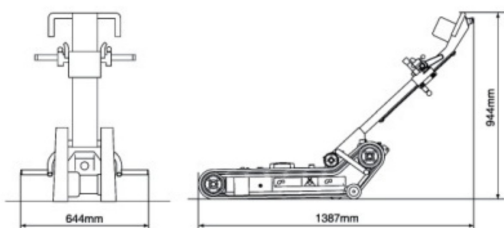
SCHEMAT TRANSPORTERA SA-S
